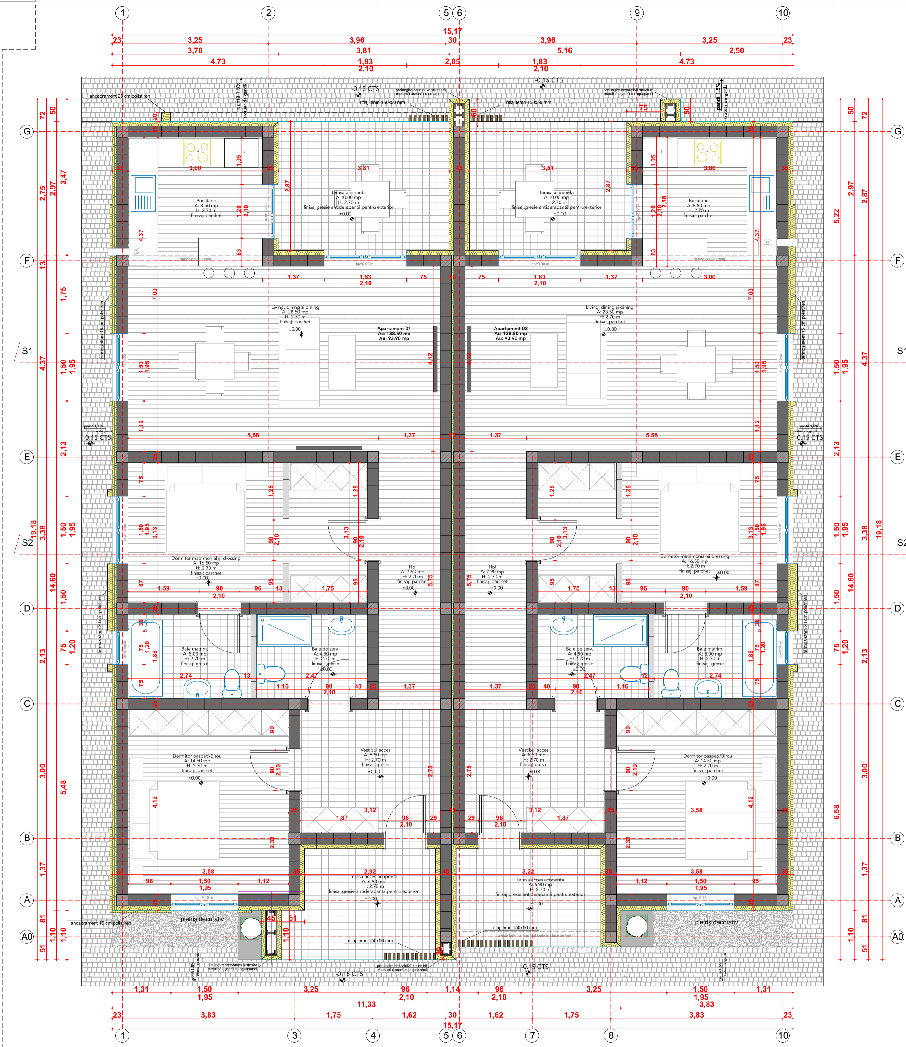
PLAN PARTER
